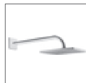
HANSAVIVA overhead shower, DN 15 0418 0240 chrome shower head square 200 x 200 mm projection: 400 mm
