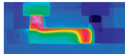
Conventional thermostat
