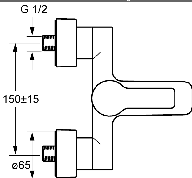
Product Drawing
