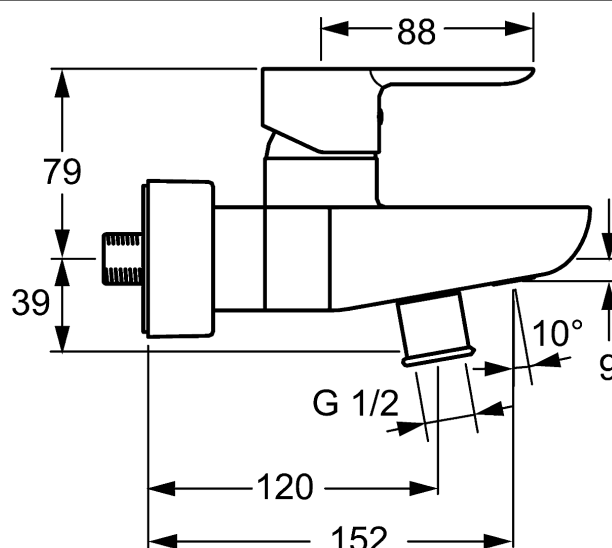
Product Drawing
